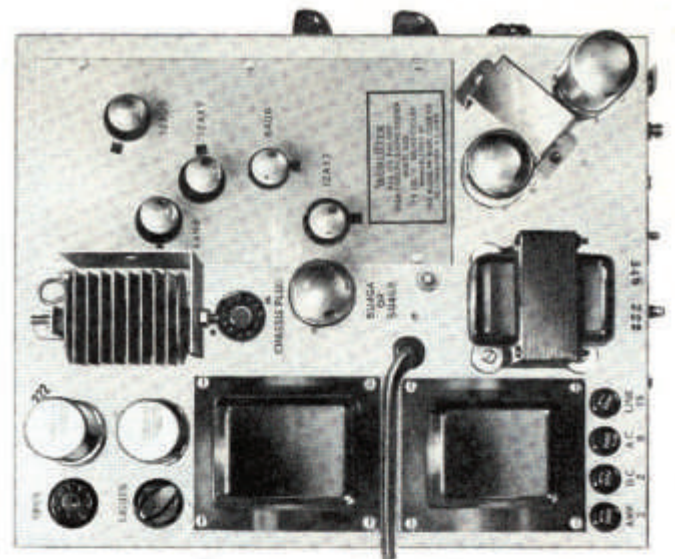
Dynatone Amplifier
